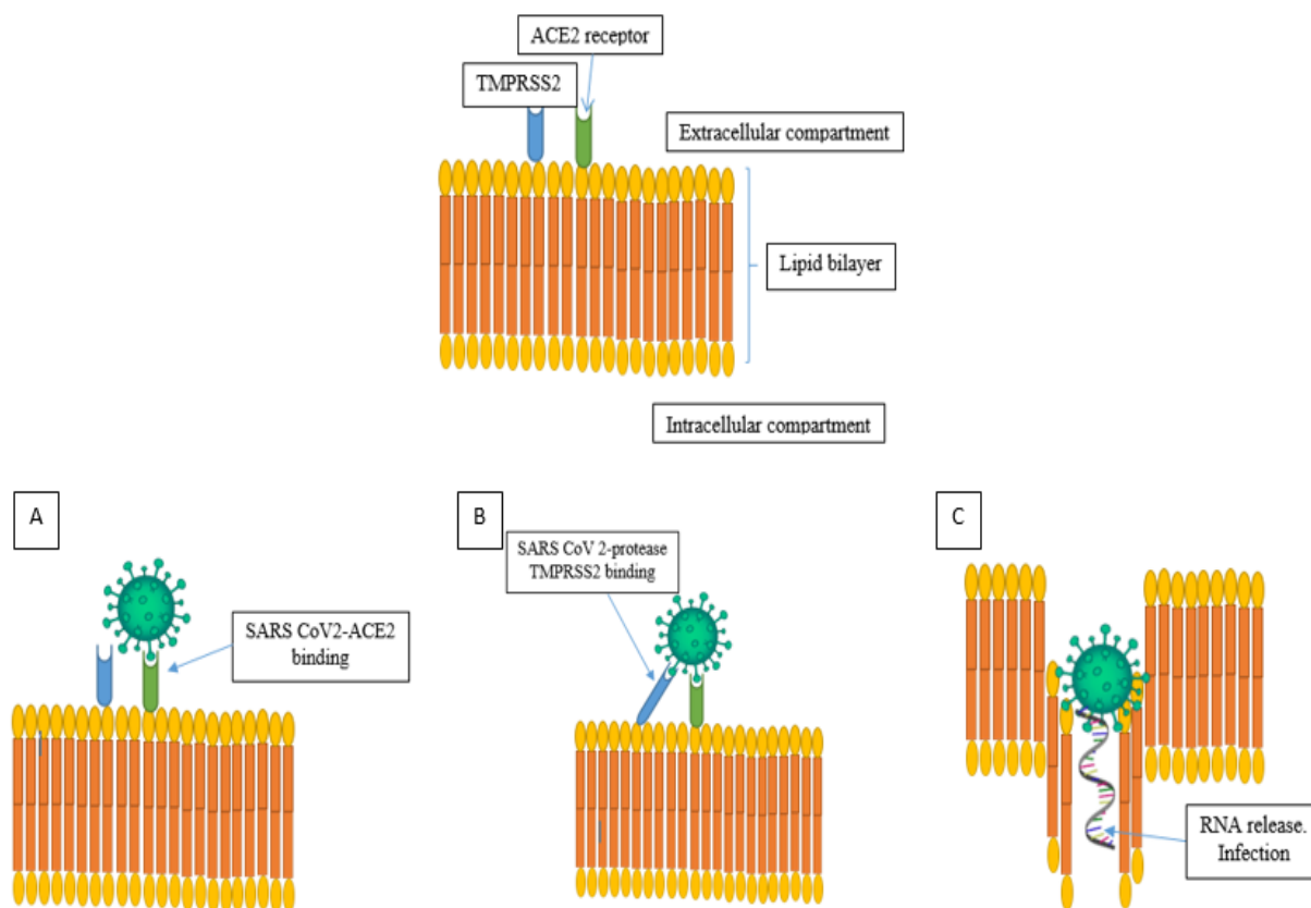
Figure 3. SARS-COV2 viral infection mechanism
